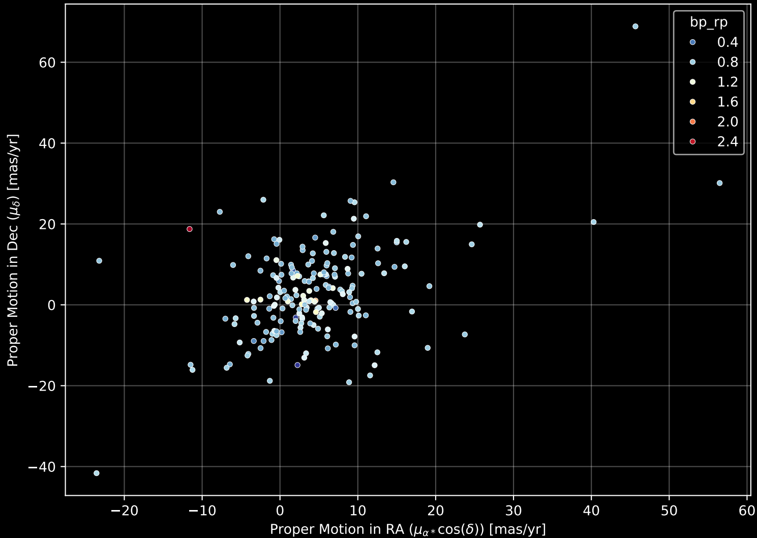
GALAH DR4 Field: [403] Proper Motion Diagram (n= 190)
