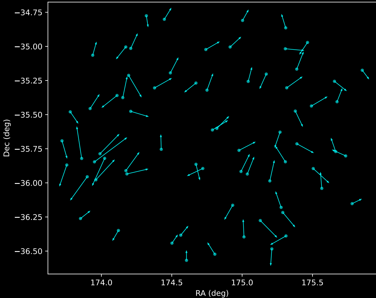
GALAH DR4 Noise Stream Proper Motion Vectors (n=70)
