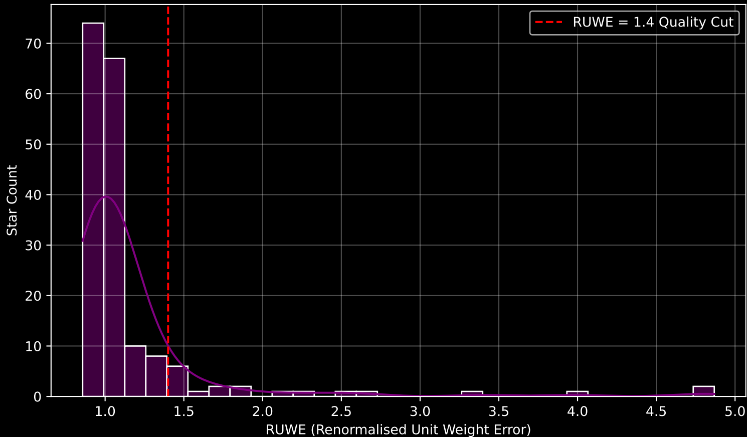
GALAH DR4 Field [403] RUWE Distribution (n= 178)
