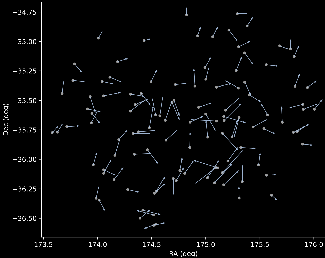
GALAH DR4 Cluster 1 Proper Motion Vectors (n=110)
