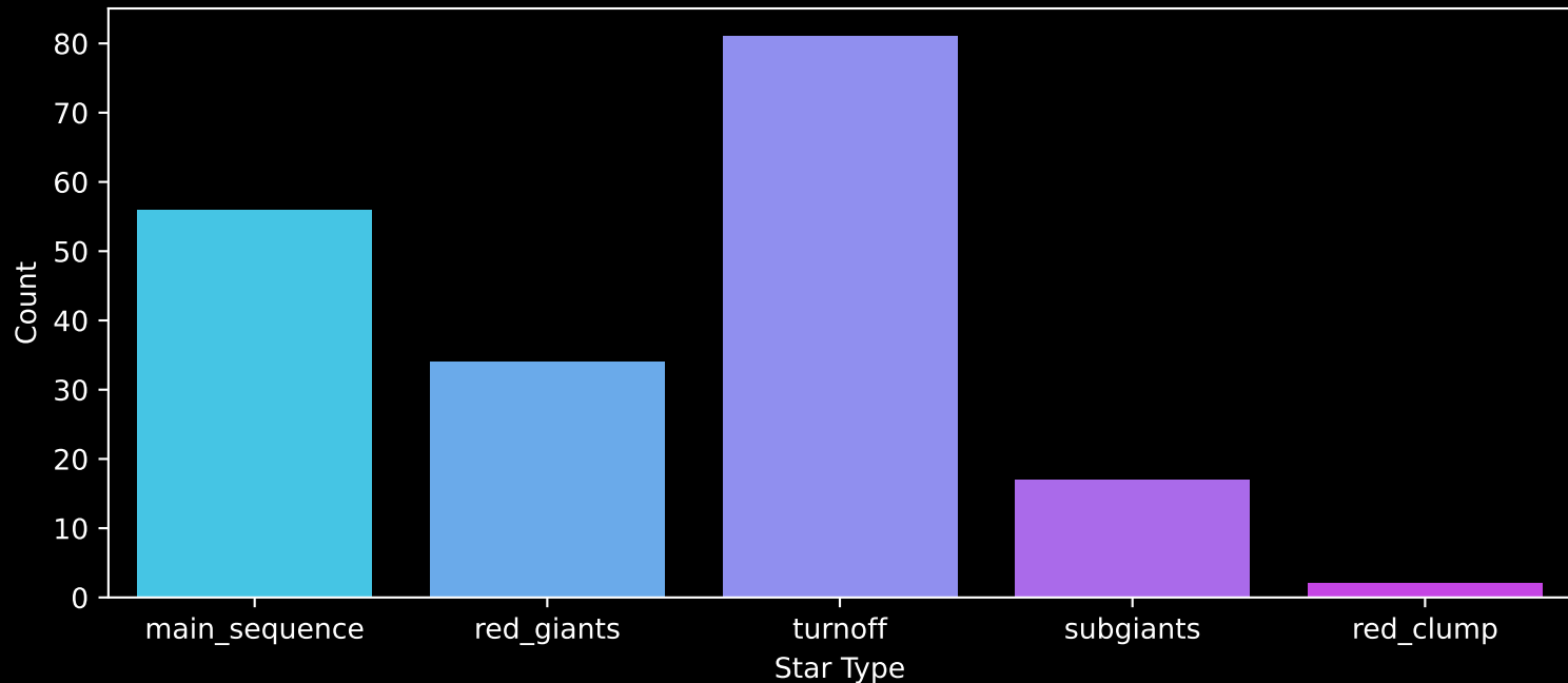
GALAH DR4 Field: [403] Count plot of Star Type
