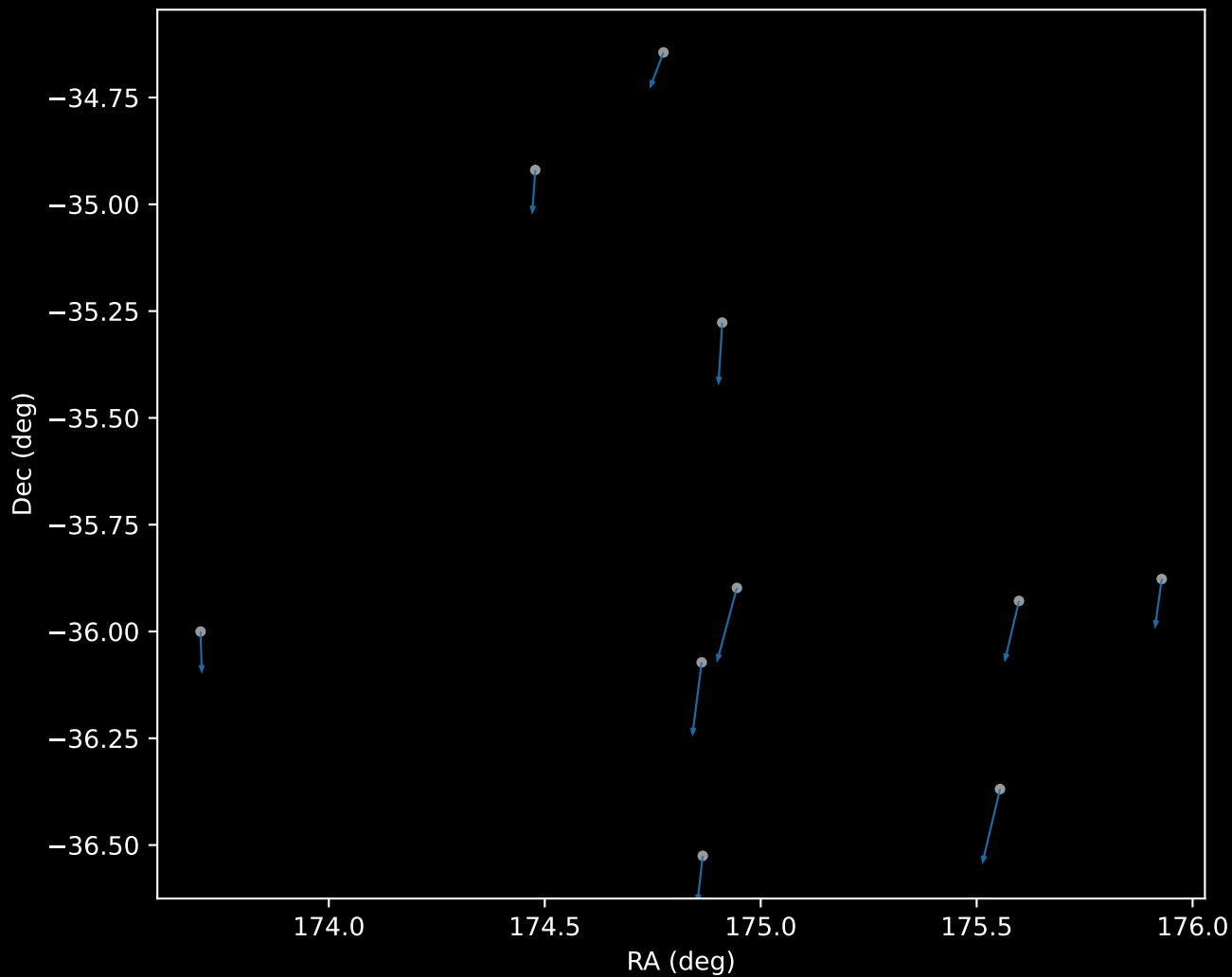
GALAH DR4 Cluster 0 Proper Motion Vectors (n=10)
